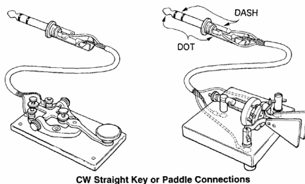
CW Straight Key or Paddle Connections
