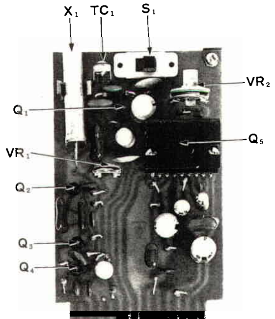
Fig. 16 AF-CALIB UNIT
