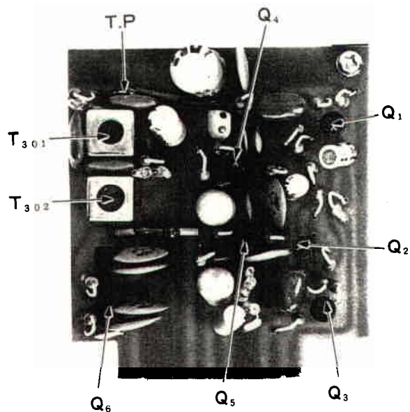
Fig. 22 FM UNIT
