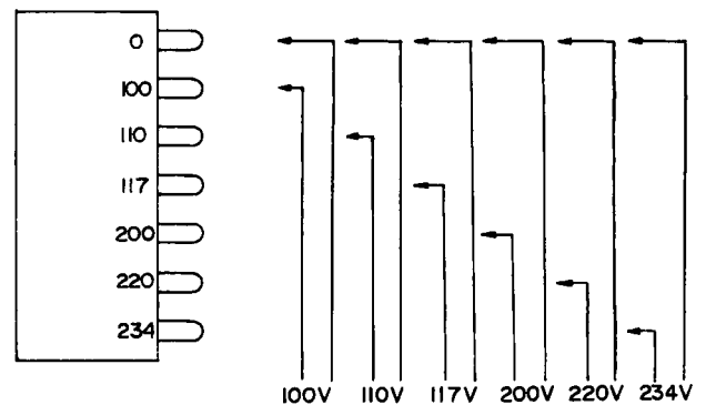
POWER TRANSFORMER PRIMARY CONNECTIONS
