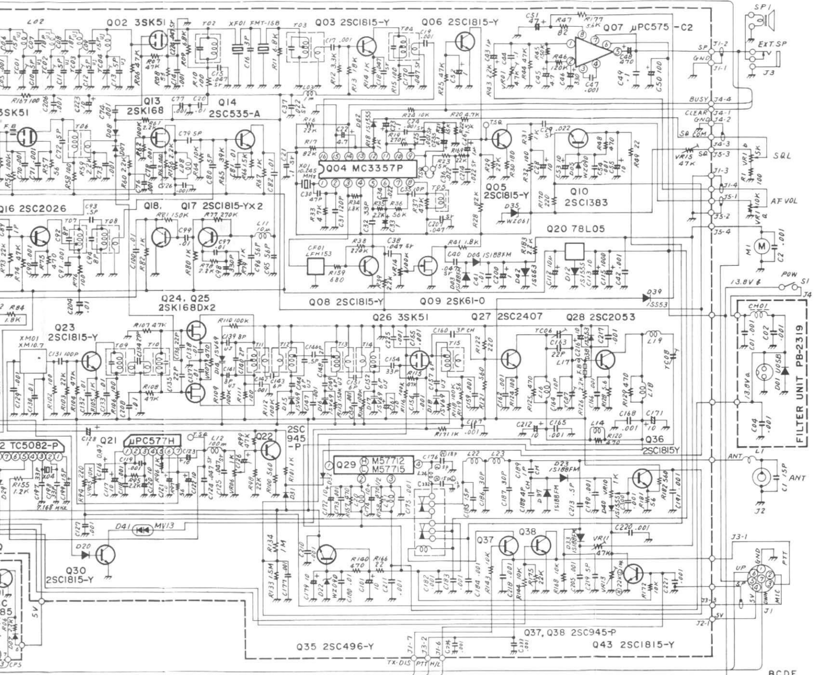
FT-230R CIRCUIT DIAGRAM
